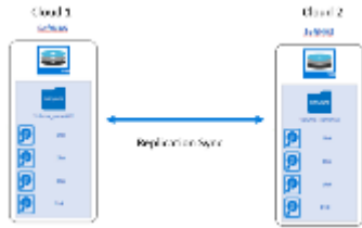
Disaster Recovery
